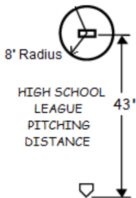
CIRCLE AREA DETAIL & PITCHING DISTANCE
